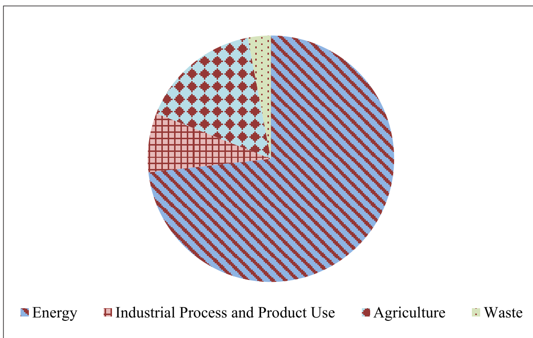
Figure 6: India’s national GHG inventory (2014)* (Gigagram)
